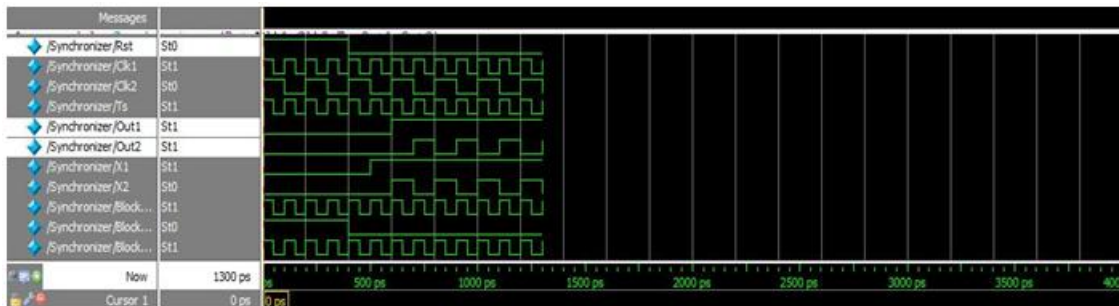
Fig.4 Synchronizer
